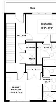
THIRD FLOOR
